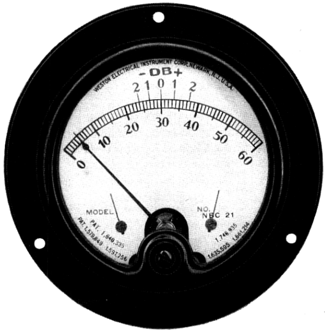
Fig. 13—Scale on 21 type volume indicator.
